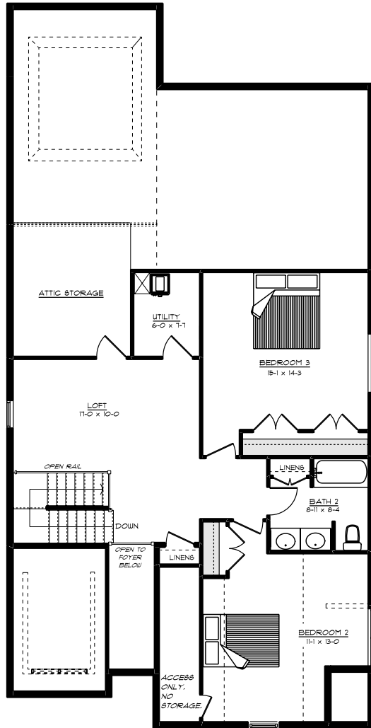
SECOND FLOOR
